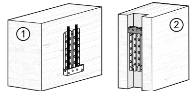
Secondary Member Through Housing
