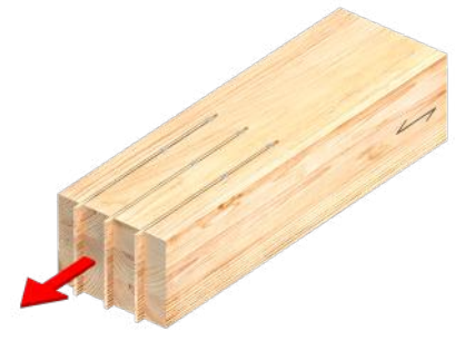
Row Shear Failure Mode
