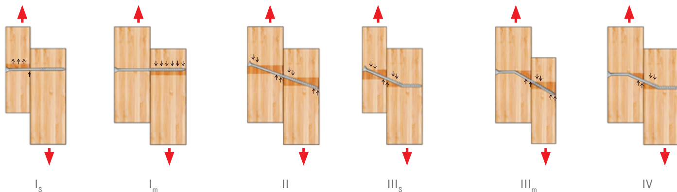
NDS Yield Modes for Two-Member Connections
