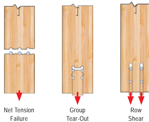
Brittle Failures in Parallel-to-Grain Loading
