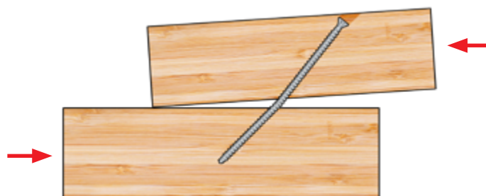
Inclined Screws in Reverse Loading
