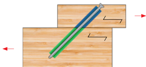
Lateral Connection with Axially Loaded Inclined Screw
