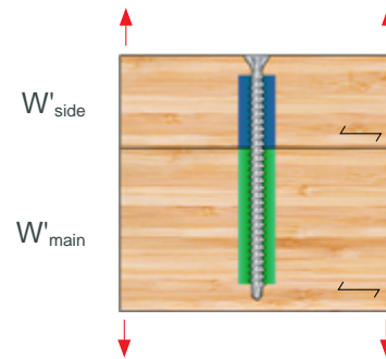
Fully Threaded Fastener in Axial Tension
