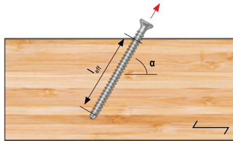
Withdrawal at Angle \alpha to the Grain
