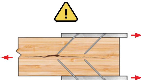
Inclined Screws in a Three-Member Connection
