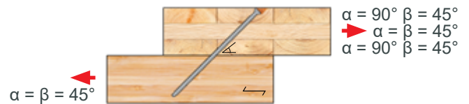
Angle Parameters for Various Configurations
