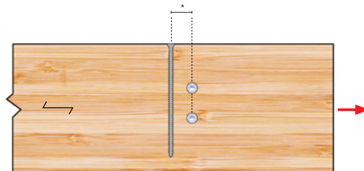
Geometry Requirements for Screws Reinforcing Bolt Connections Loaded Parallel-to-Grain
