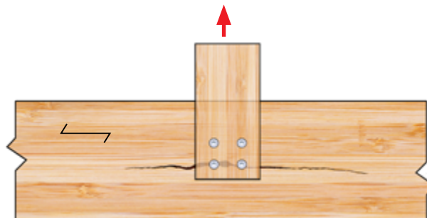
Splitting Failure in Perpendicular-to-Grain Loading
