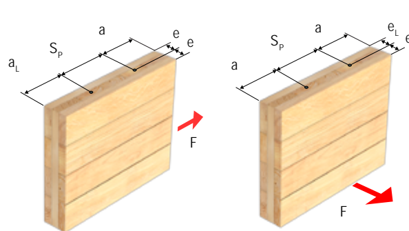
Fasteners in Narrow Edge
