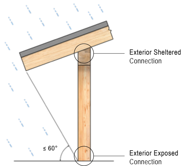
Sheltered and Exposed Connections
