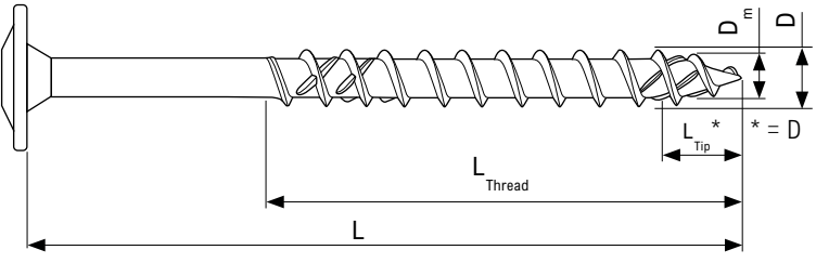
ASSY SK 4.0 - 1/4" [6 mm] DIAMETER
