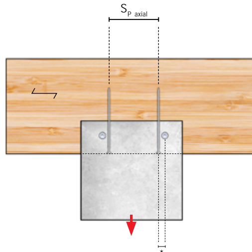
Geometry Requirements for Screws Reinforcing Bolted Connections Loaded Perpendicular-to-Grain
