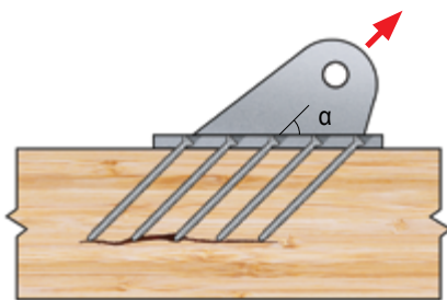
Block Shear Failure in Inclined Steel-to-Wood Connections
