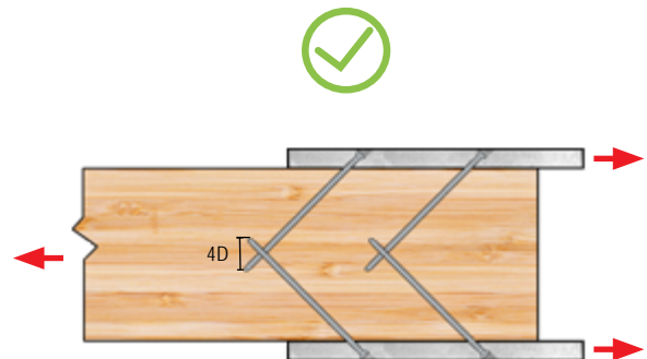
Inclined Screws in a Three-Member Connection
