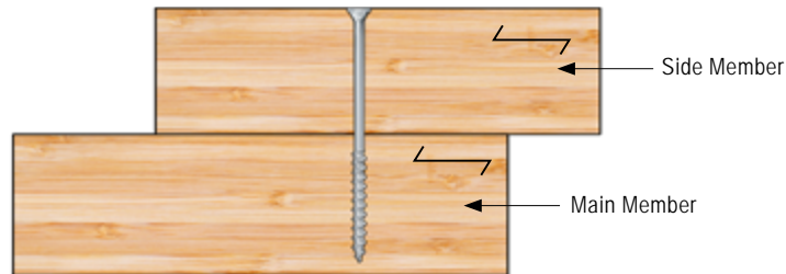
Two-Member Connection
