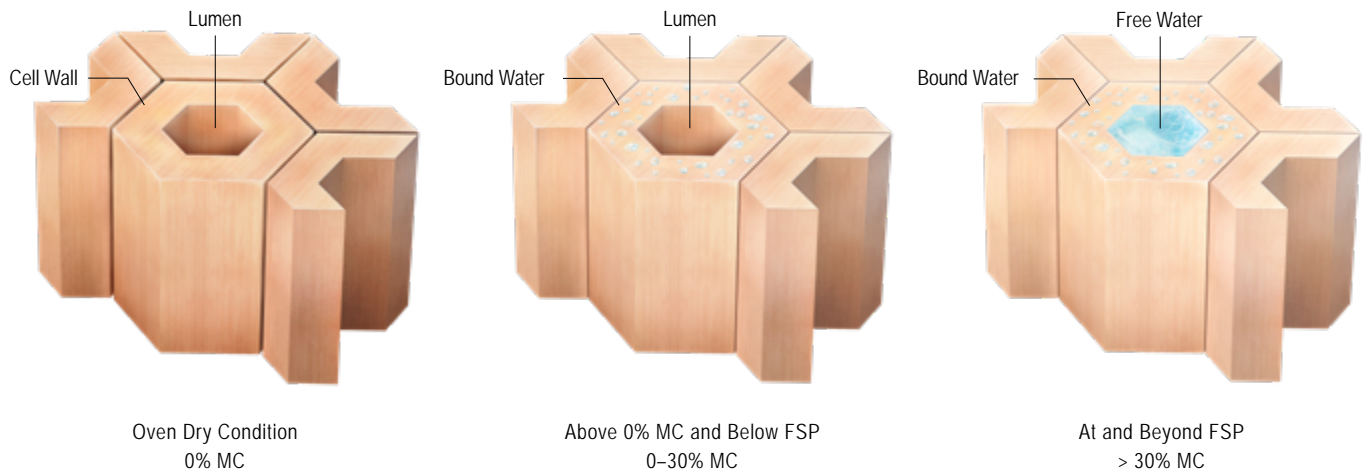
Water Movement in Wood Cells
