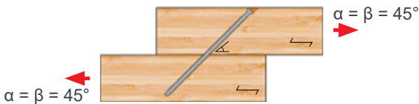
Angle Parameters for Various Configurations
