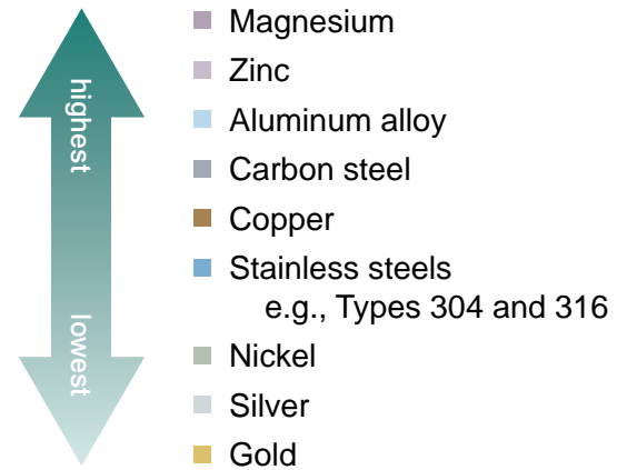
Galvanic Series of Metals and Alloys
