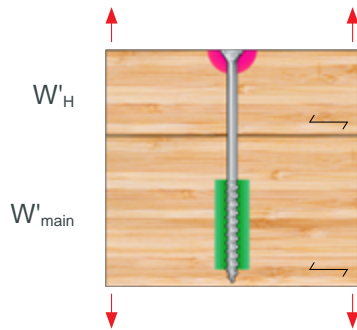
Partially Threaded Fastener in Axial Tension
