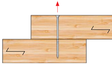
Tensile Connection
