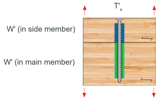
Fully Threaded Fastener in Axial Tension
