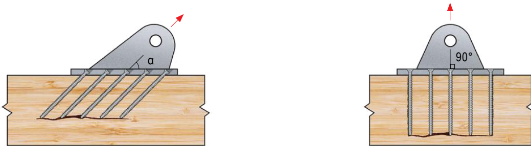
Splitting Failure Perpendicular to Grain in Steel-to-Wood Connections
