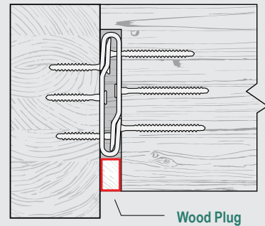
Wood Plug
