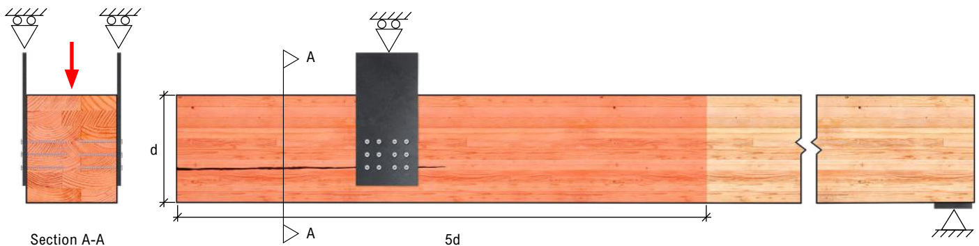
Figure C.6 - Splitting of Beam Supported Near its End
