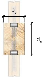
Hangers on Opposing Faces of a Rectangular Column
