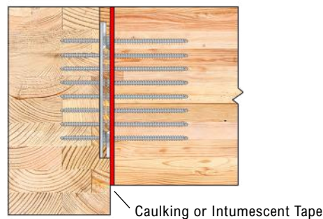
Figure A.6 - Fire-Resistant Joint
