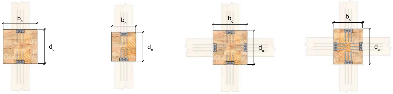
Hangers on Opposing Faces of a Square Column
