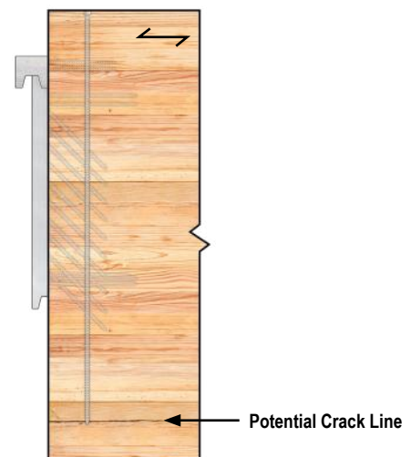
Figure C.5 - Effective Threads of Reinforcing Screw Does Not Extend to Bottom of Member
