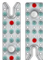
RICON S VS 200 x 60
