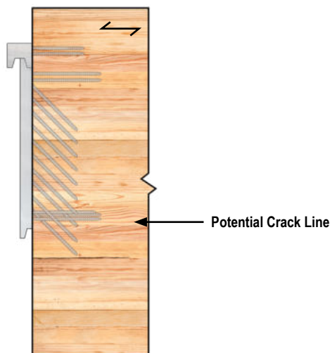
Figure C.4 - Lowest Inclined Fastener in Beam Hanger Does Not Support Bottom of Member
