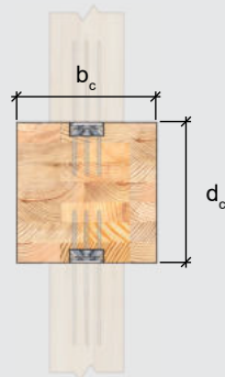
A Hangers on Opposing Faces of a Square Column
