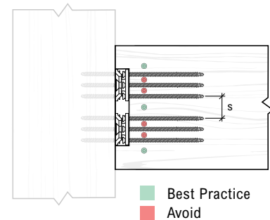
Figure C.11 - Reinforcing Screw Placement for Avoiding Screw Collisions
