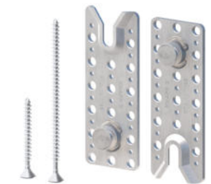
MTC-FTC RICON S VS Plates
