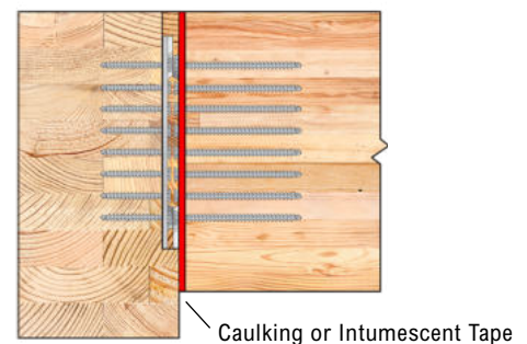
Figure A.6 - Fire-Resistant Joint for GIGANT, RICON S VS, and MEGANT
