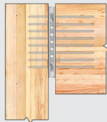
Surface-Mounted
