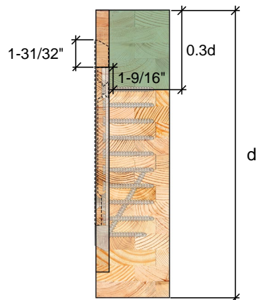
Primary Beam
