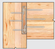
Housed in Primary Member (Column)
