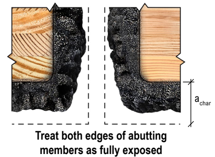
Figure A.3b - Char Contraction for Exposed Members
