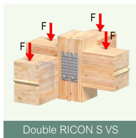
Wood Beam-to-Steel
