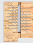
Housed in Secondary Member (Joist or Purlin)
