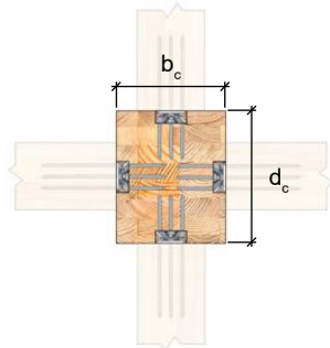
Hanger on Each Face of a Rectangular Column
