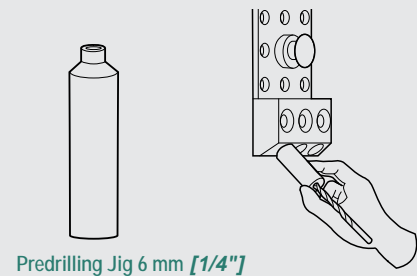
Predrilling Jig 6 mm [ 1/4 in. ]
