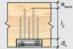
Housed
