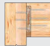
Housed in Secondary Member (Joist or Purlin)
