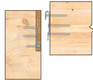
GIGANT Concealed in the Primary Member
