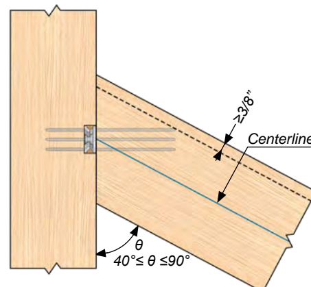
Top View: Joist to Beam or Column Connection
