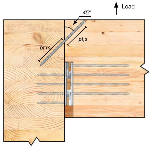
Example of Toe Screw Installation
