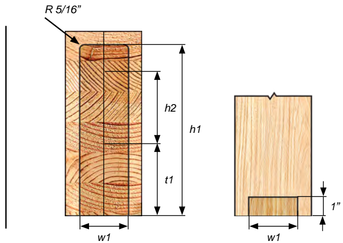
Section View
