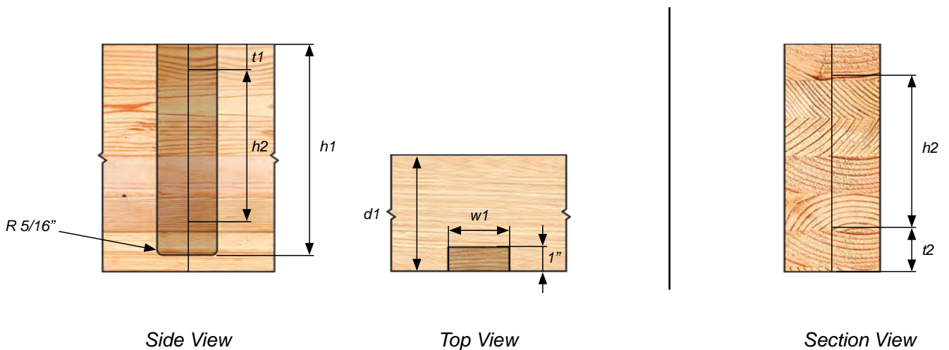
Primary Member
