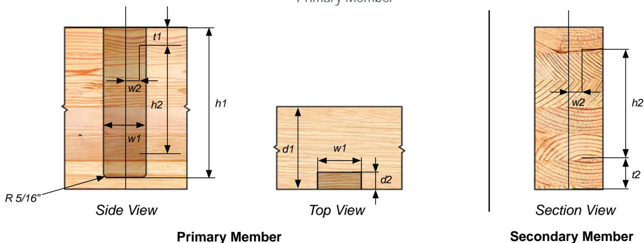
MEGANT Concealed in the Primary Member
