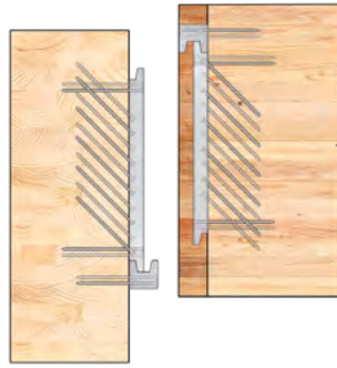
MEGANT Concealed in the Secondary Member
